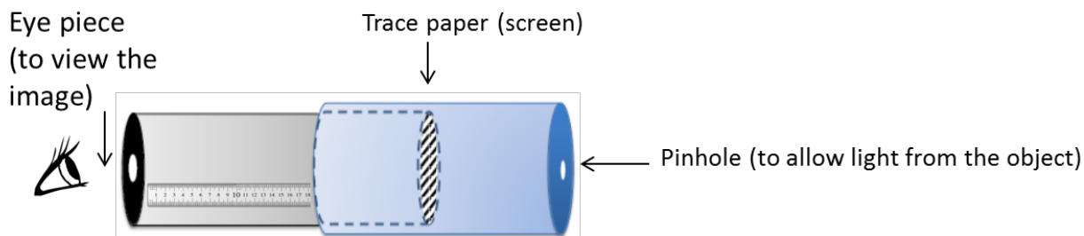
Figure 1 Schematic of pinhole camera that can acts as a measuring device
